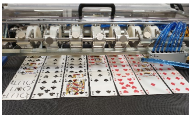
All In – die-cutting solutions with Swiss precision, BOGRAMA presents the versatility of its rotary die-cutting machine.
